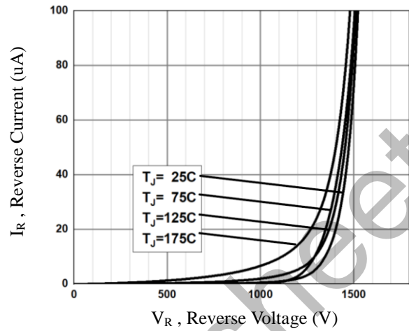
Fig.2 Reverse Characteristics
