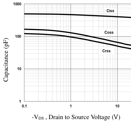
Fig.6 Capacitance Characteristics
