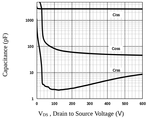
Fig.7 Capacitance Characteristics
