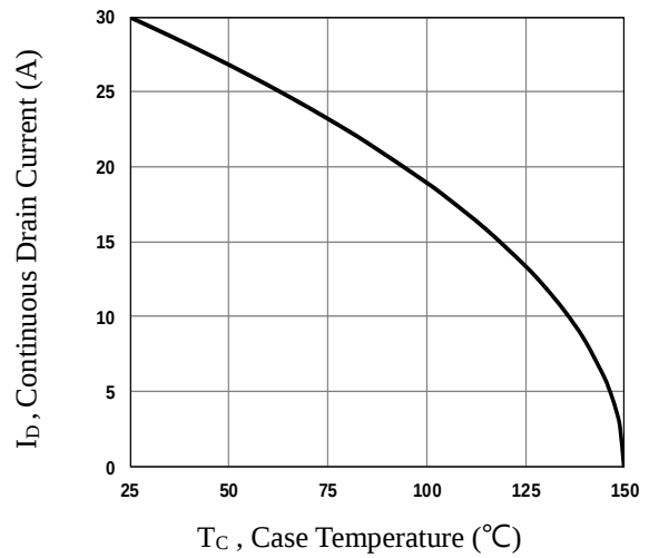
Fig.8 Continuous Drain Current vs. T_C
